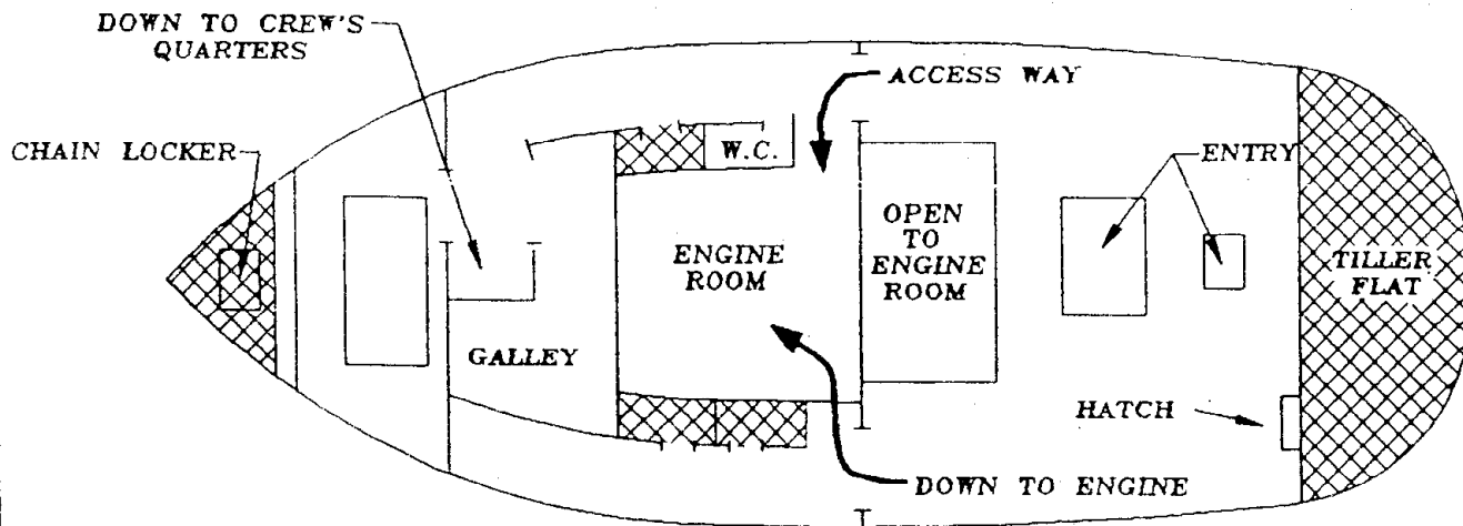
PLAN - LEVEL "A"
