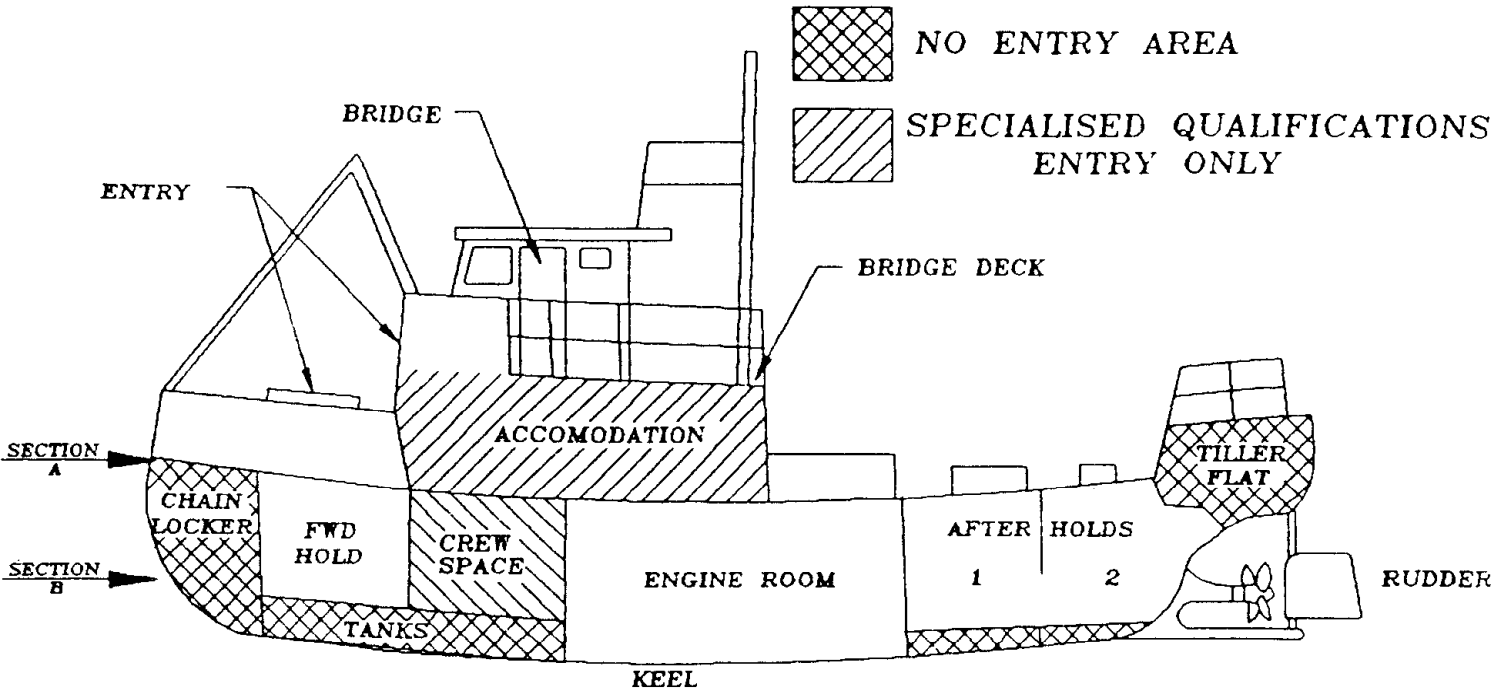
VESSEL ELEVATION
